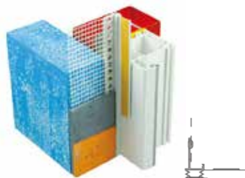
644600 accordion PVC reveal profile with mesh for 9 mm render
