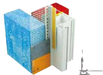
644810 reveal profile DYNAMIK PVC with mesh / dimensions 9 mm
